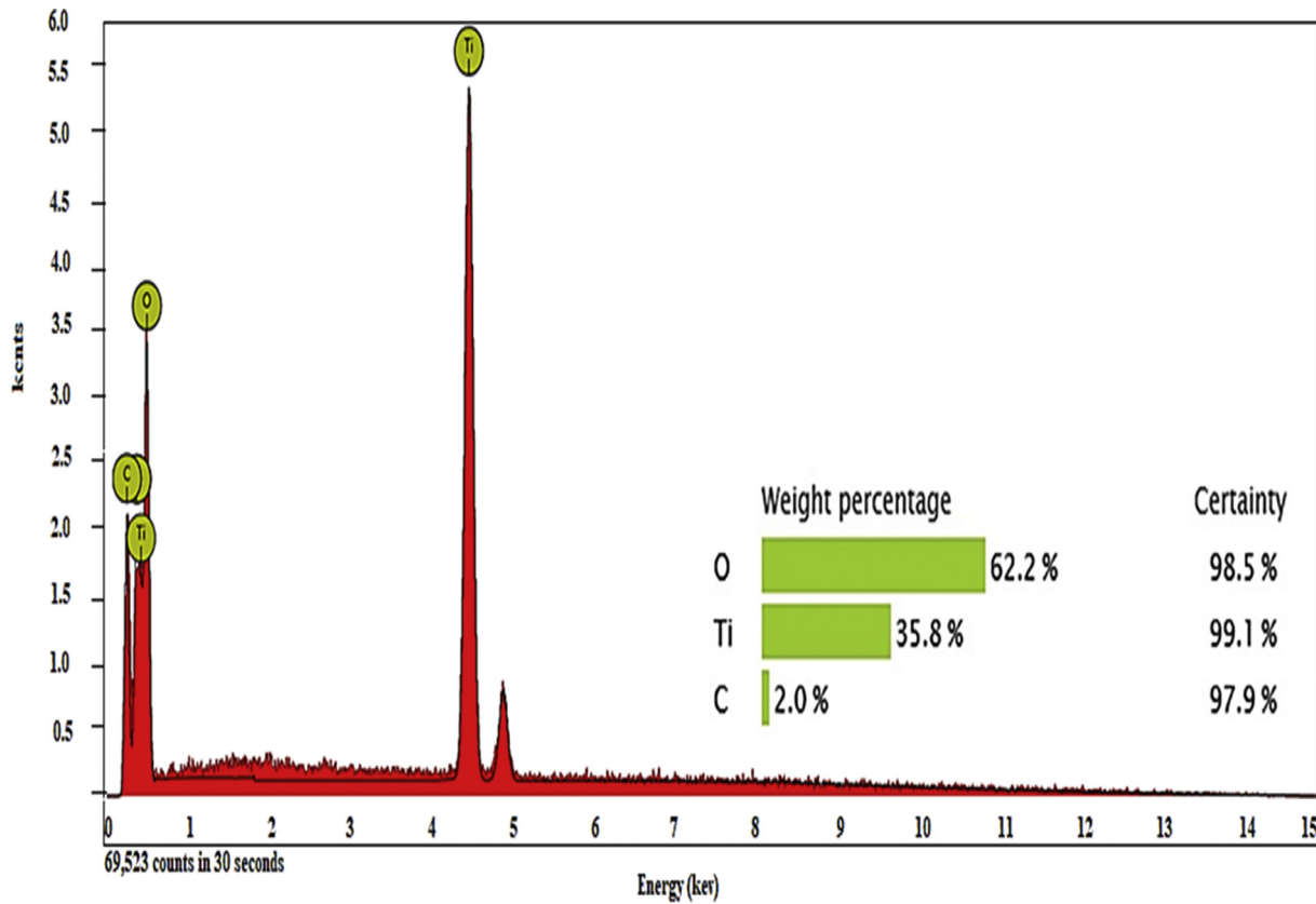
Figure 4. EDX analysis of the TiO 2 nanoparticle (Source: Gill et al. [21]).
