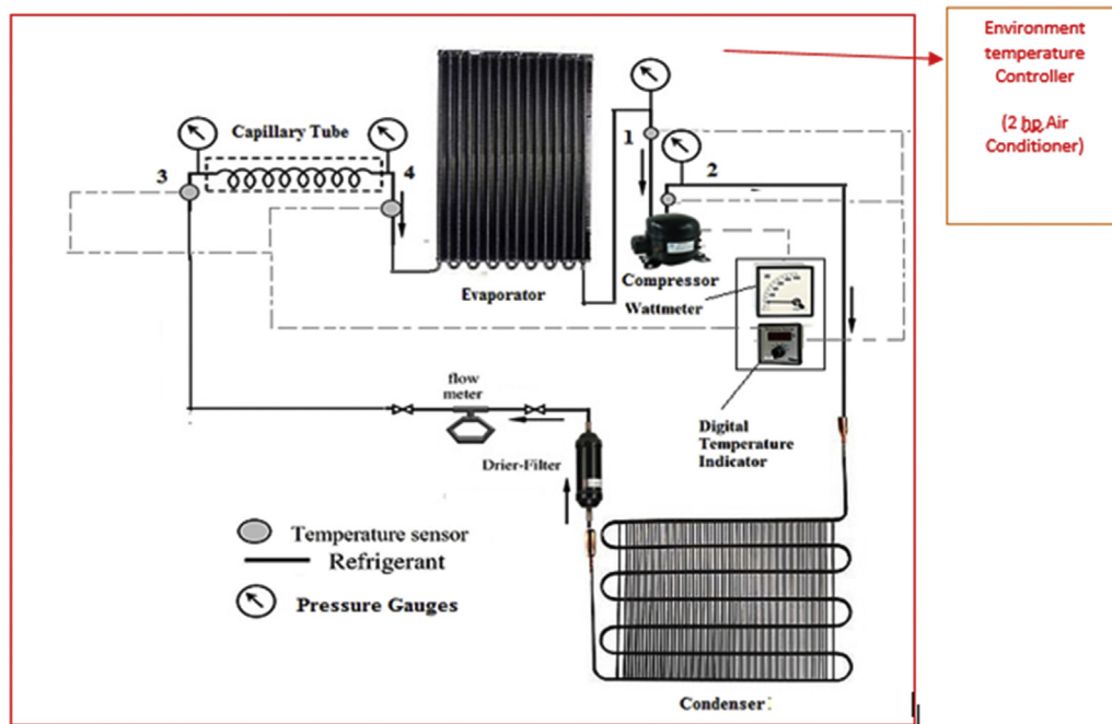
Figure 1. Schematic of the refrigeration system (Source: Gill et al. [21]).
