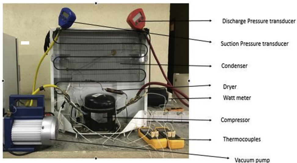
Figure 2. Experimental Setup of Test Rig (Source: Ohunakin et al. (2018)).
