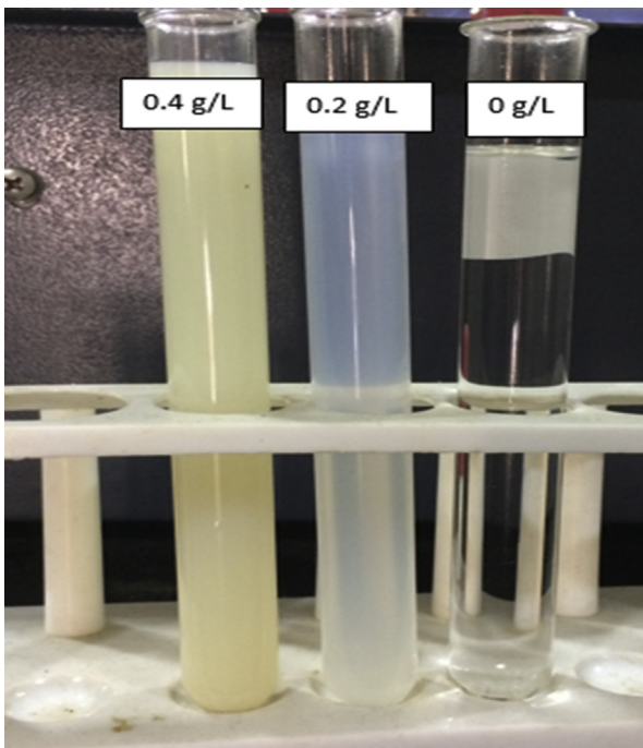
Figure 5. Ultrasonicated nanolubricants After 24 h.
