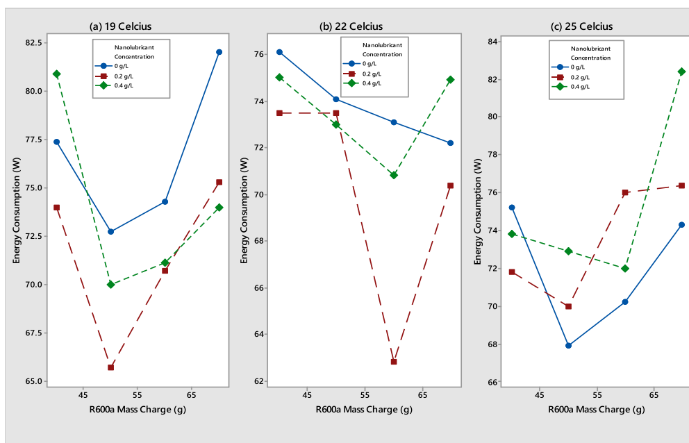
Figure 9. (a–c): Variation of energy consumption across 19, 22 and 25 °C ambient temperatures.
