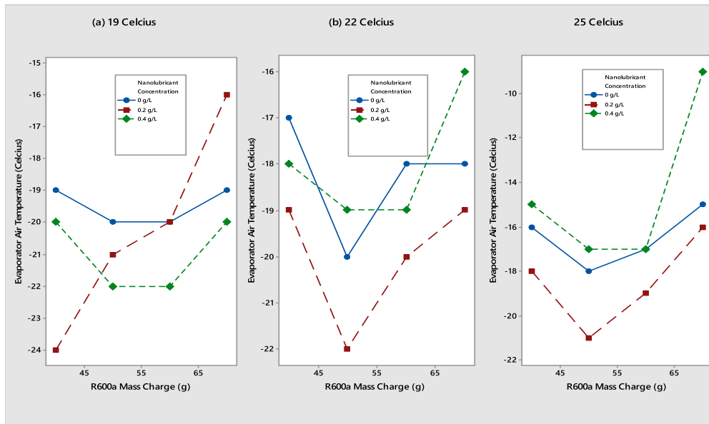
Figure 8. (a–c): Variation of evaporator air temperature across 19, 22 and 25 °C ambient temperatures.
