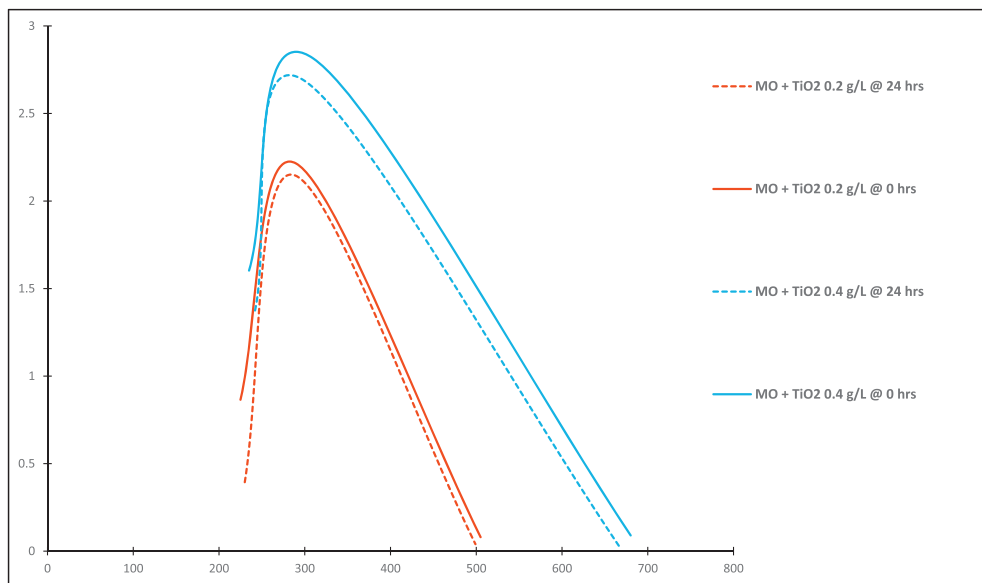
Figure 7. Variation of the nanolubricant absorbance.
