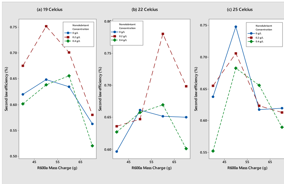
Figure 10. (a–c): Variation of coefficient of performance across 19, 22 and 25 °C ambient temperatures.
