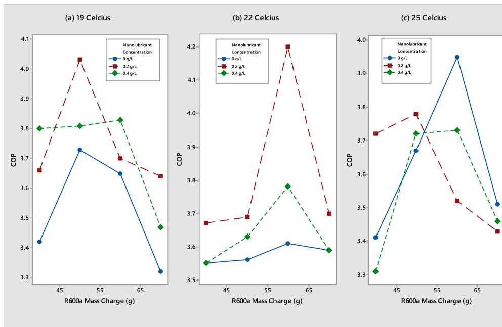
Figure 11. (a–c): Variation of second law efficiency across 19, 22 and 25 °C ambient temperatures.
