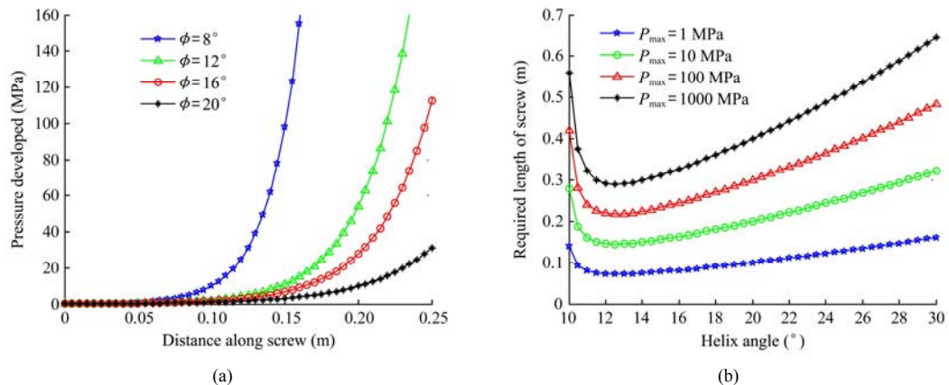
Figure A4 Effect of the helix angle on: (a) pressure build-up; (b) required screw length
