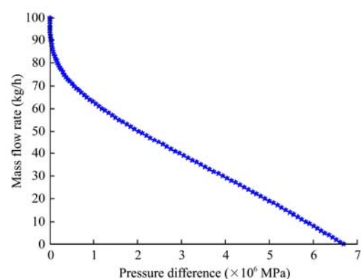
Figure 4 Plot of the mass flow rate with pressure difference of a tapered screw extruder biomass briquetting machine.
