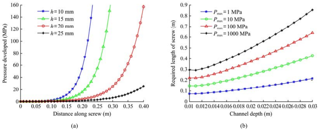
Figure A3 Effect of the channel depth on: (a) pressure build-up; (b) required screw length
