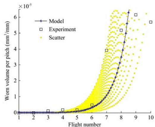
Figure 6 Comparison of the predicted screw wear of the briquetting machine from analytical model with experimental results from Ghimire and Shrestha (2014).
