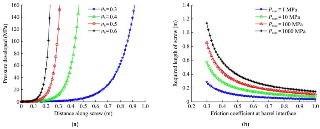
Figure A1 Effect of friction coefficient at the barrel-material interface on: (a) pressure build-up; (b) required screw length
