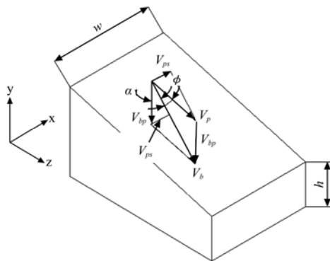
Figure 3 Velocities of the plug flowing through a tapered screw extruder channel (Ojolo et al., 2015)
