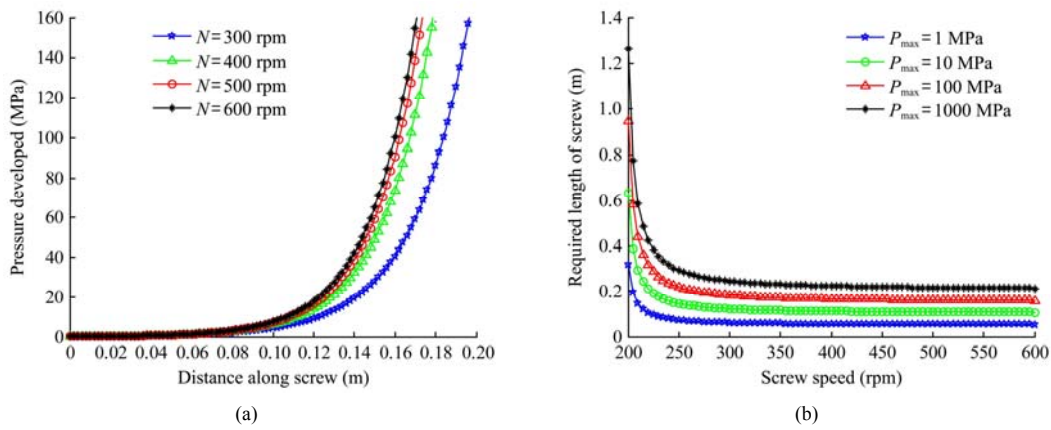
Figure A5 Effect of screw speed on: (a) pressure build-up; (b) required screw length
