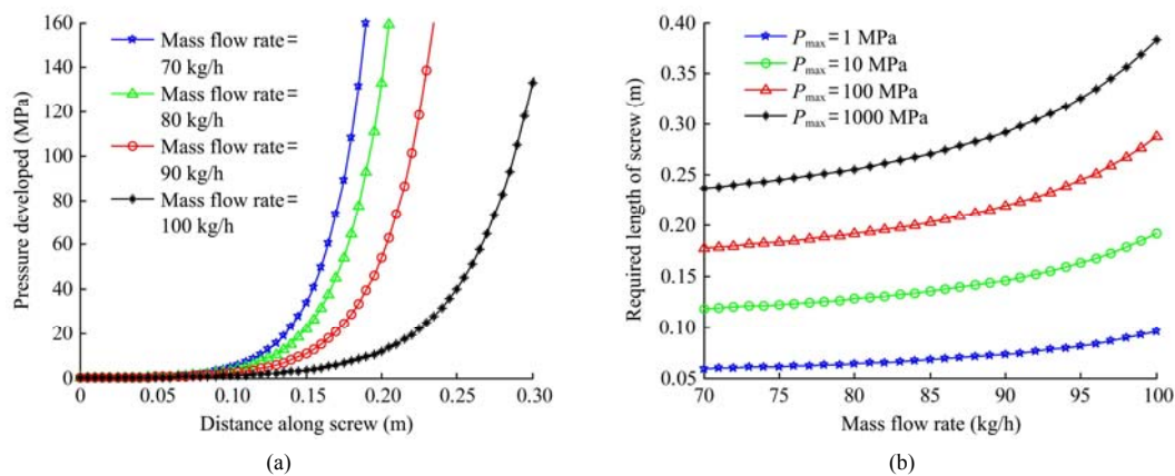
Figure A6 Effect of mass flow rate on: (a) pressure build-up; (b) required screw length
