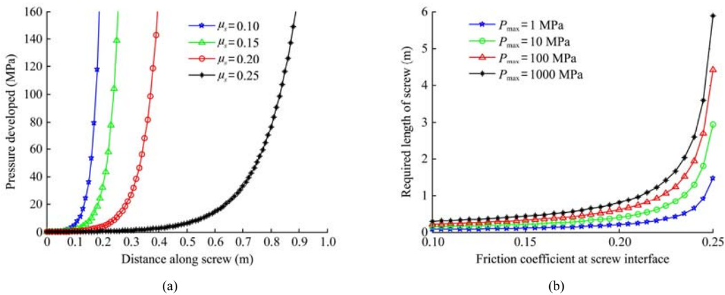
Figure A2 Effect of friction coefficient at the screw-material interface on: (a) pressure build-up; (b) required screw length
