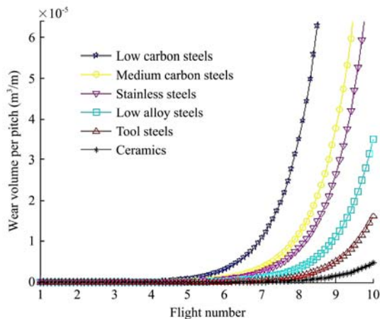
Figure 8 Influence of material of screw on the worn volume of the screw of a biomass briquetting machine
