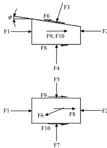
Figure 2 Forces acting on elemental slice of plug in inclined channel (Ojolo et al., 2015)
