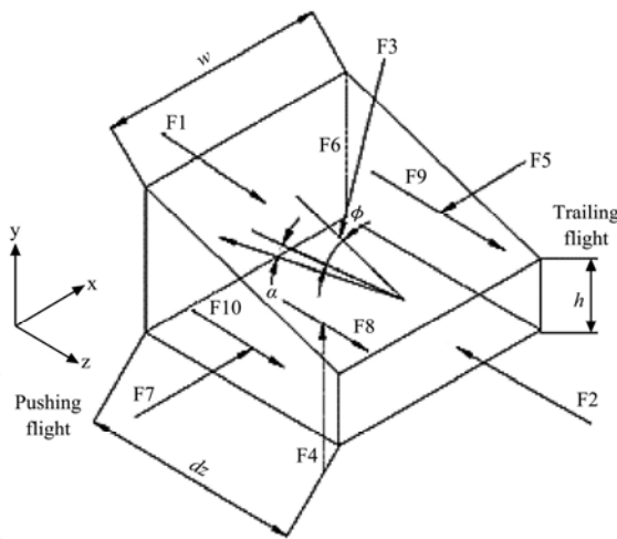
Figure 2 Forces acting on elemental slice of plug in inclined channel (Ojolo et al., 2015)
