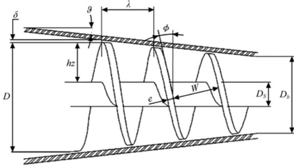
Figure 1 Schematic of the tapered screw with geometric description
