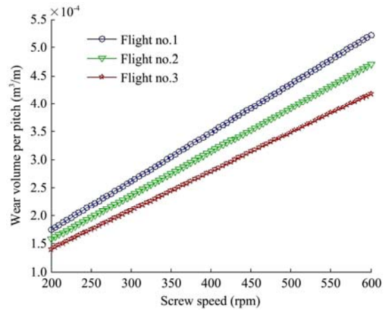
Figure 7 Relationship between the screw speed and wear volume of the screw extruder biomass briquetting machine for the first three flights from the briquetting die.
