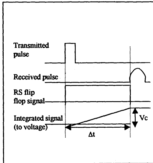
Figure 3: Distance measurement using integration method
