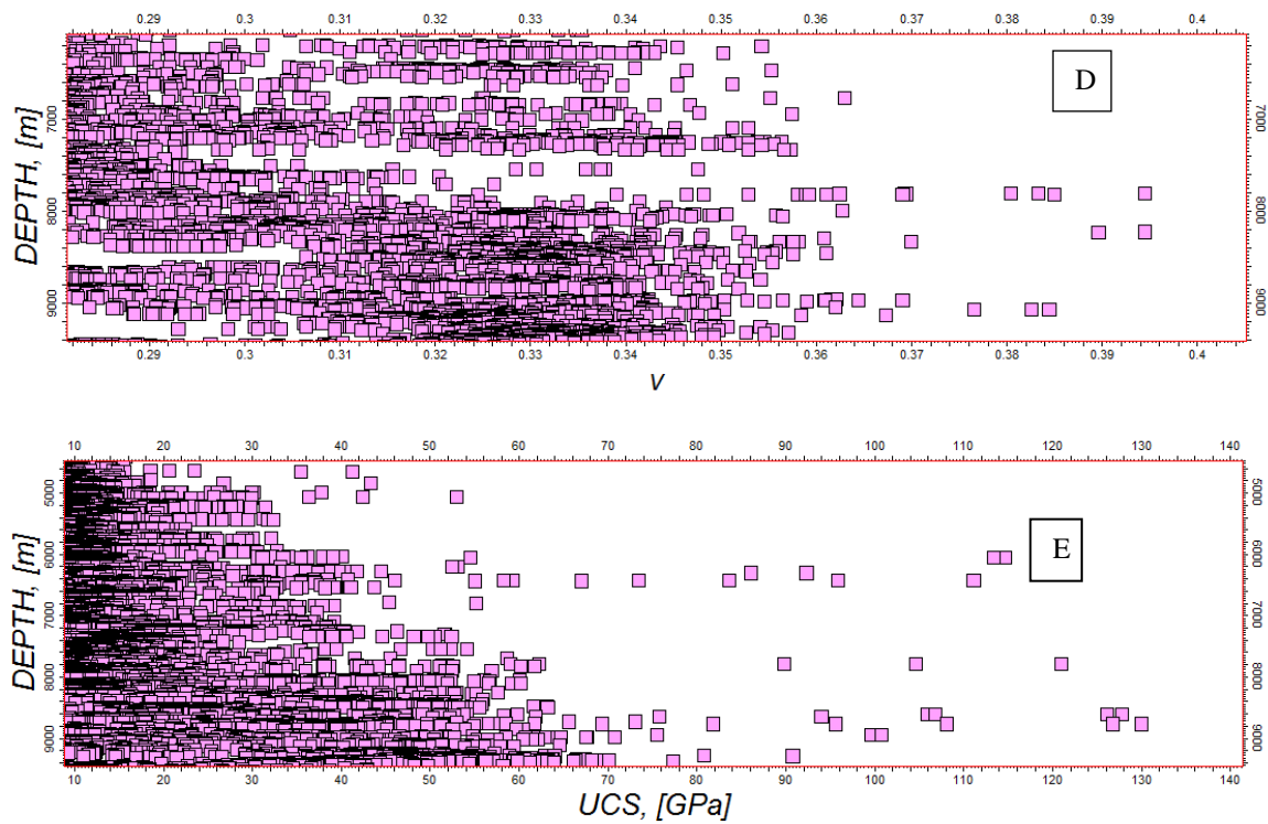
Fig 8b: Relationship between depth and the elastic and inelastic properties of the reservoir for Well Law 2; (D) Poisson's Ratio [v] (E) Unconfined Compressive Strength [UCS]
