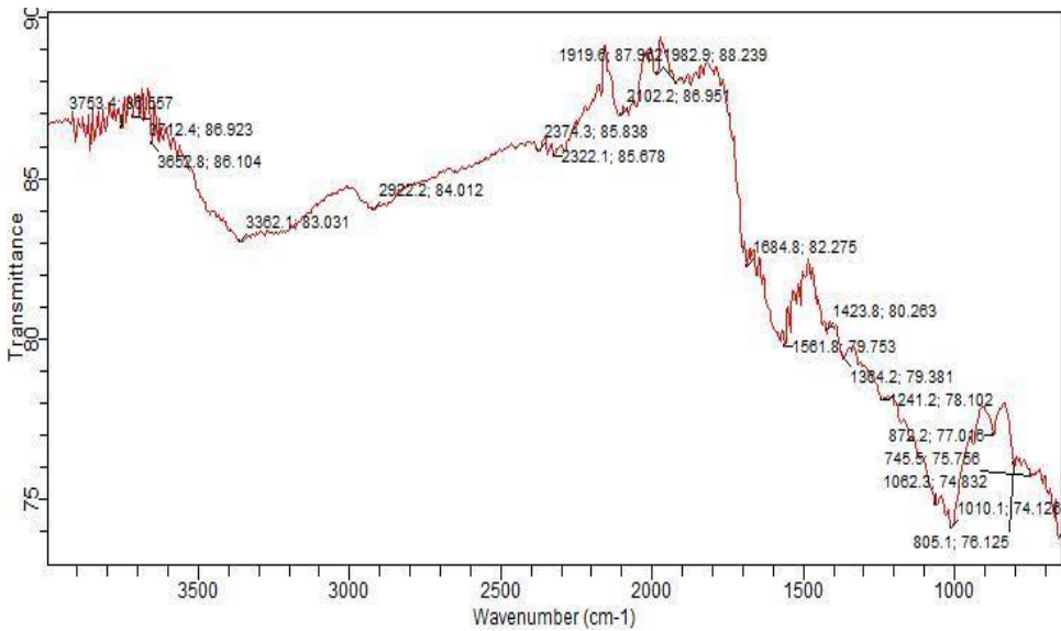
Figure 5: FTIR Spectra of RTA
