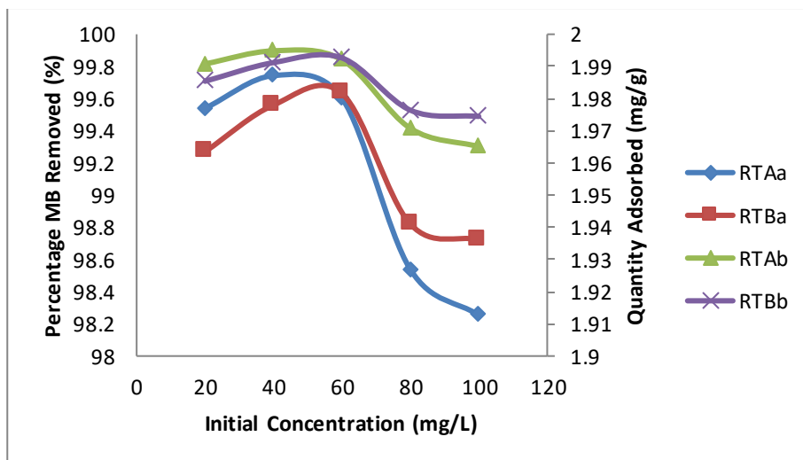
Figure 12: Effect of initial concentration on adsorption capacity of RTA and RTB
