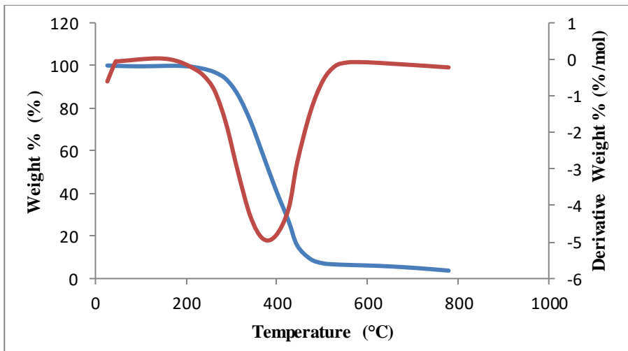
Figure 7: TGA/DTG curves for RTR
