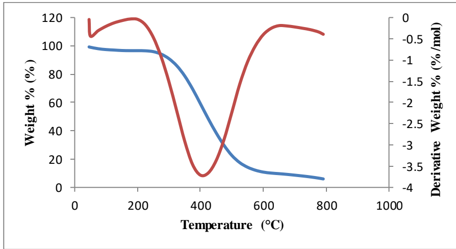
Figure 9: TGA/DTG curves for RTB
