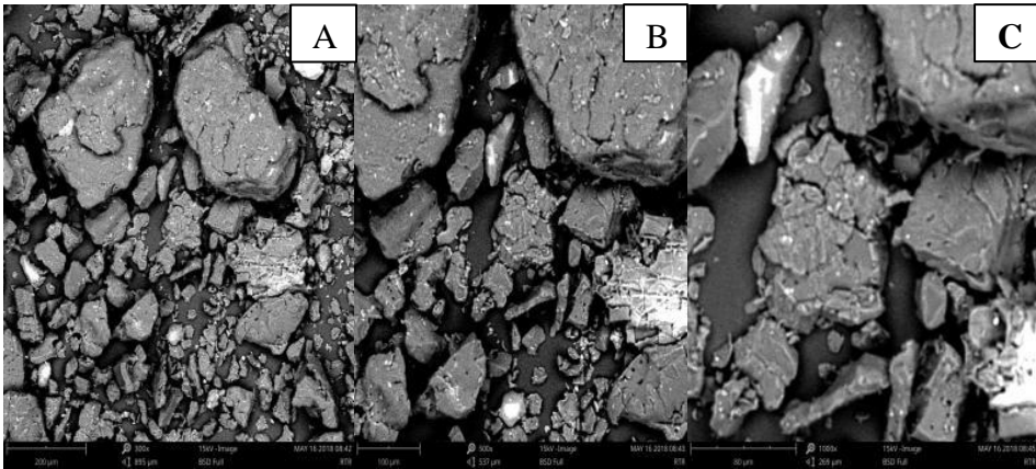
Figure 1: SEM images of RTR at 300x (A), 500x (B) and 1000x (C)
