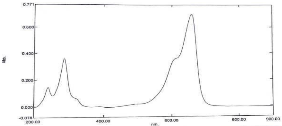
Figure 10: Absorption Curve of Methylene Blue as a function of Wavelength.
