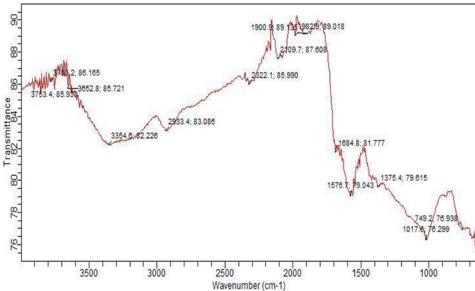
Figure 6: FTIR Spectra of RTB
