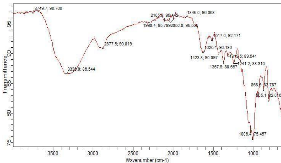
Figure 4: FTIR Spectra of RTR
