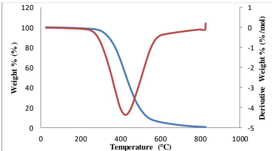
Figure 8: TGA/DTG curves for RTA
