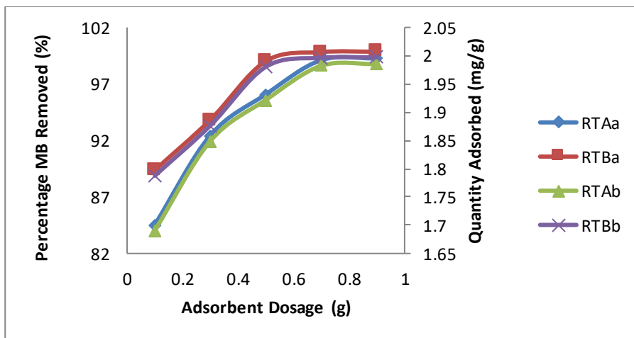
Figure 11: Effect of dosage on adsorption capacity of RTA and RTB
