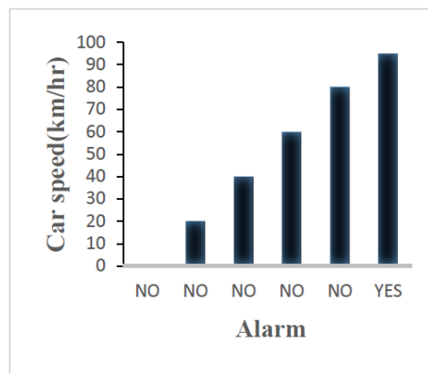
Fig. 9. Histogram of car speed against alarm for Honda Accord and Toyota Corolla.
