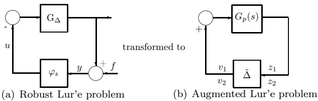
Using LFT, the system in Fig. 6(a) is transformed into Fig. 6(b)
