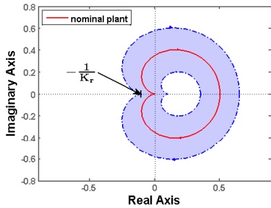
Fig. 5. Robust Nyquist Plot
