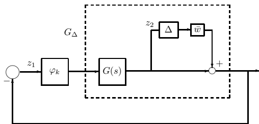
Fig. 12. Robust Lur'e for Output Multiplicative Uncertainty
