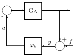
Fig. 3. The Robust Lur'e problem.
