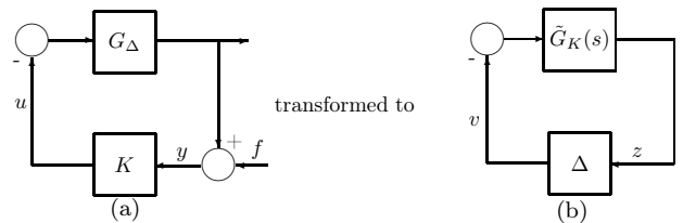
Fig. 4. The Uncertain System.
