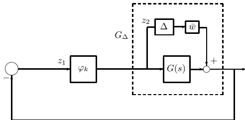
Fig. 8. Robust Lur'e for Additive Uncertainty
