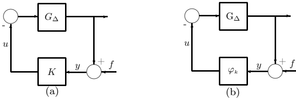
Fig. 7. Robust Kalman Conjecture (RKC).
