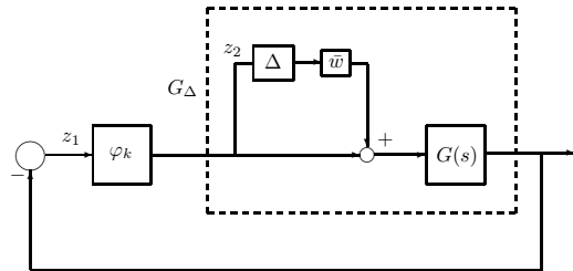
Fig. 10. Robust Lur'e for Input Multiplicative Uncertainty
