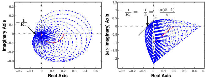
Fig. 11. Robust Nyquist and Robust Popov Plots
