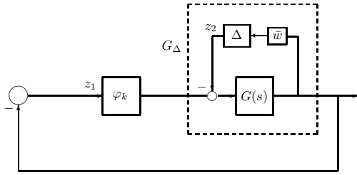
Fig. 14. Robust Lur'e for Feedback Uncertainty
