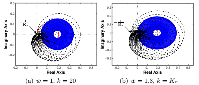
The robust Zames-Falb plots are scaled by 1500.
