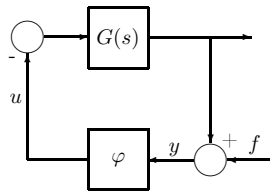
Fig. 1. The Lur'e Structure.
