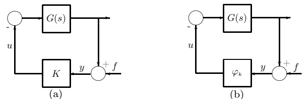
Fig. 2. The Absolute Stability Conjecture.
