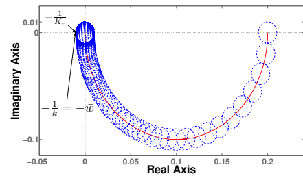
Fig. 9. Robust Nyquist Plot
