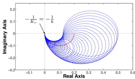
Fig. 15. Robust Nyquist Plot
