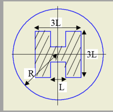
Fig. 5. The die profile (plan view) from round to H-section
