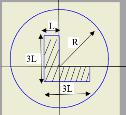
Fig. 4. The die profile (plan view) from round to L-section
