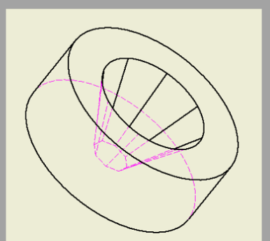
Fig. 11. Streamlined die for extrusion of octagonal section
