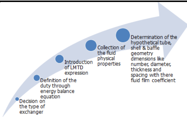
Fig. 8: Modeling Procedure
