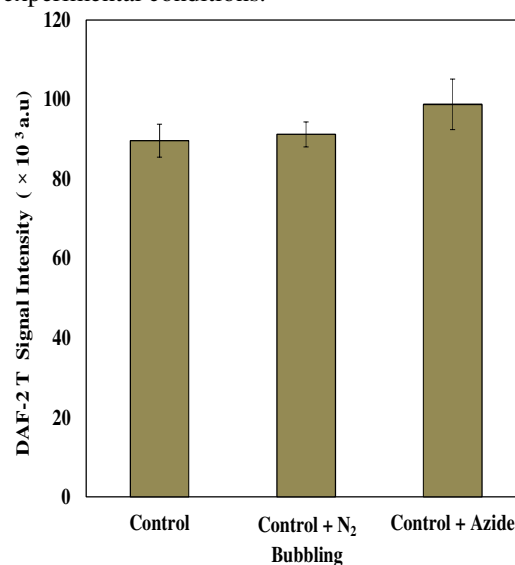
Figure 2b: The signal intensity of DAF-2T generated by the irradiation of 10 \mu\text{M} \text{NO}_2^- with 5 \mu\text{M} DAF-2 for 20 min in air-saturated solution (control), with the addition of 0.5 \text{ mM} sodium azide, and when the solution was purged with \text{N}_2 for 30 min prior to irradiation. Each experiment was conducted in triplicate.
