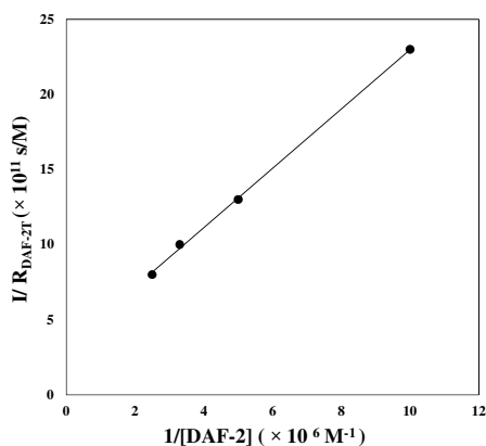
Figure 4. Graph for the calculation of the rate constant for the reaction of DAF-2 with NO\bullet using the alternate competition kinetics method. A plot of reciprocal of DAF-2T photo-formation rate ( 1/R_{DAF-2T} ) and inverse of the concentration of added DAF-2 ( 1/[DAF-2] ) in Milli-Q water. [NO_2^-]: 10 \mu M , [DAF-2]: (0.1- 0.4 \mu M) ; [Hb]: 0.1 \mu M . The values for the y-intercept and slope are 3.45 \times 10^{11} s/M and 1.93 \times 10^5 s respectively, correlation coefficient ( r^2 ) = 0.993.
