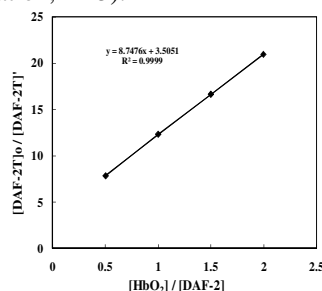
Figure 3: Graph for the calculation of the rate constant for the reaction of DAF-2 with \text{NO}\cdot radical using the competition kinetics method, correlation coefficient ( r^2 ) = 0.999.
