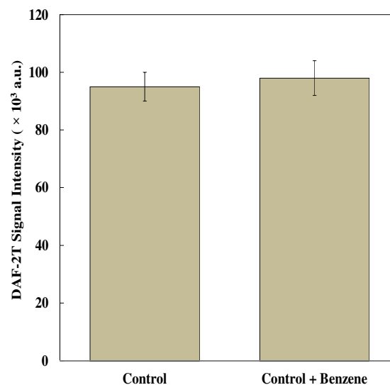
Figure 2a: The signal intensity of DAF-2T produced by the irradiation of 10 \mu\text{M} \text{NO}_2^- and 5 \mu\text{M} DAF-2 for 20 min in air-saturated solution (control) and with the addition of 1.2 mM benzene. Each experiment was conducted in triplicate.
