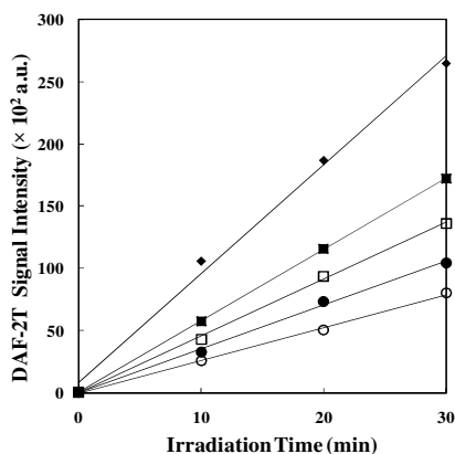
Figure 2c Signal intensities of DAF-2T produced by the irradiation of 10 \mu\text{M} \text{NO}_2^- and 0.5 \mu\text{M} DAF-2 in Milli-Q water with and without \text{HbO}_2 as a function of irradiation time. Closed diamonds: 0 \mu\text{M} \text{HbO}_2 ; closed rectangles: 0.1 \mu\text{M} \text{HbO}_2 ; open rectangles: 0.2 \mu\text{M} \text{HbO}_2 ; closed circles: 0.3 \mu\text{M} \text{HbO}_2 ; open circles: 0.4 \mu\text{M} \text{HbO}_2 .
