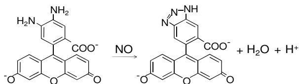
Fig.1 Structures of DAF-2 and DAF-2T
