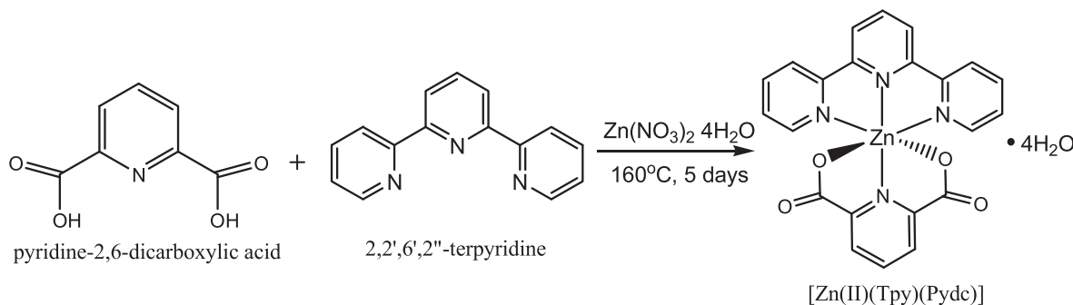
Scheme 1. Synthesis of [\text{Zn}(\text{II})(\text{Tpy})(\text{Pydc})\cdot 4\text{H}_2\text{O}] .
